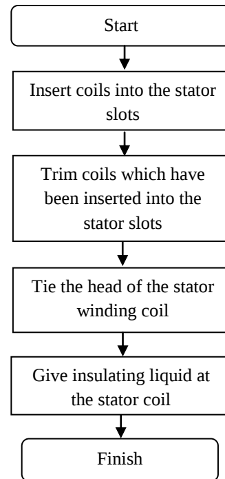
Figure 3 a. Flow chart of the making of stator windings b. Flow chart of the installation of stator windings
